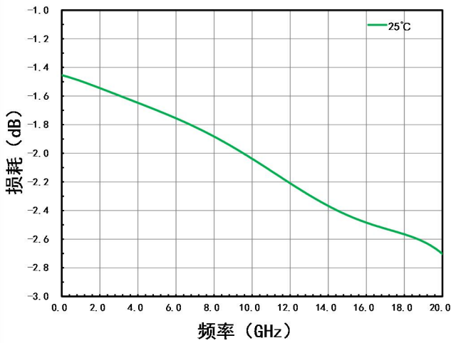
损耗 VS. 零态 25°C
